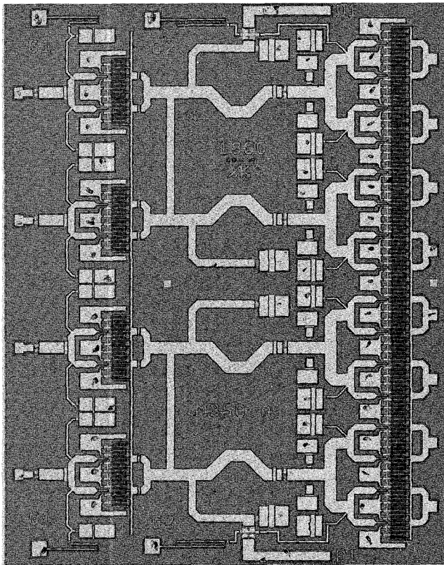
Figure 1. Micrograph of Ku-Band MMIC
